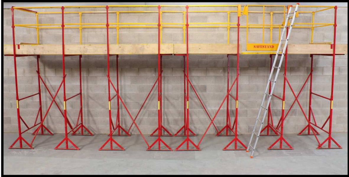
8m run, shown raised to full extension; 2.210m platform
